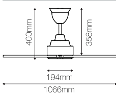
RCF-VENTO42-5B 42"
