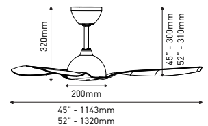
RCF-FREDD045/52-3B 45"/52"
